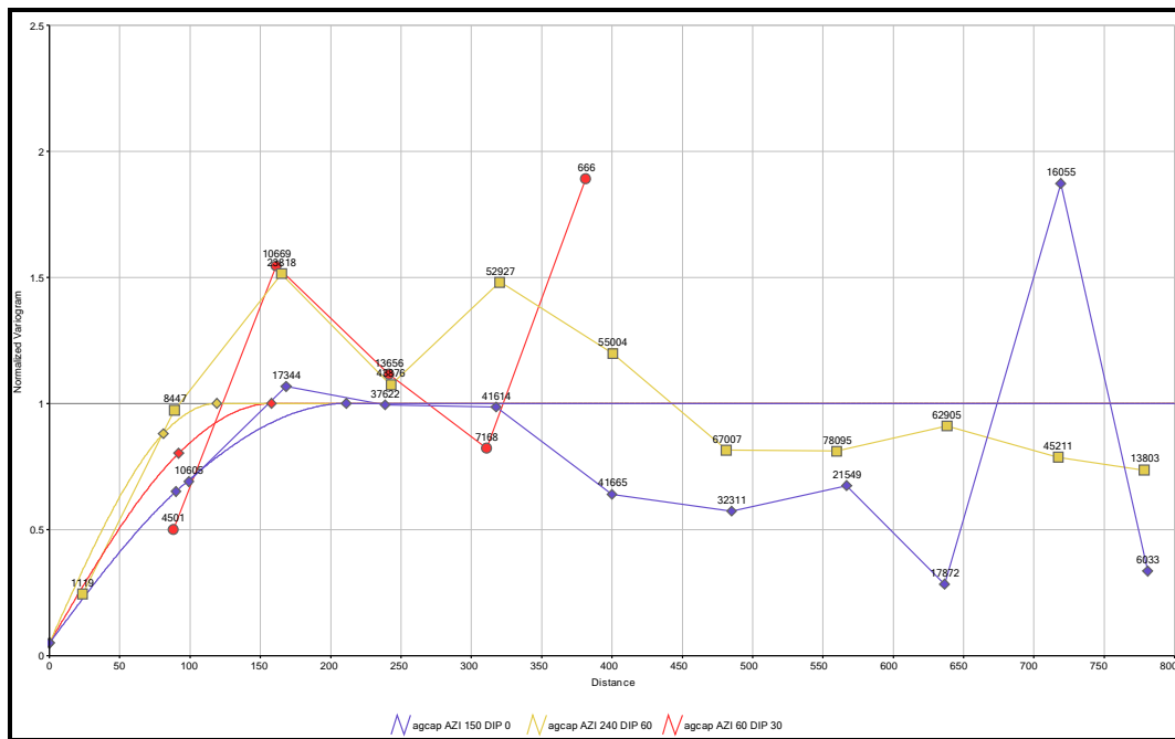
Figure 14.33 Bear Creek Hanging-Wall Zone Silver Variogram
