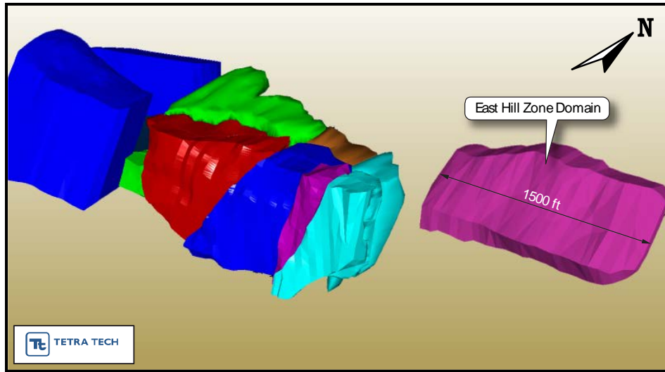
Figure 14.11 Oblique View East Hill Zone
