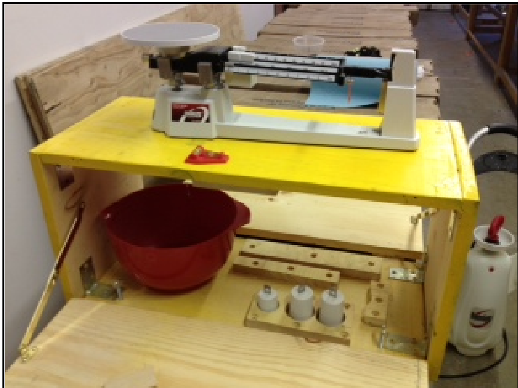
Figure 14.1 Specific Gravity Measurement Scale
