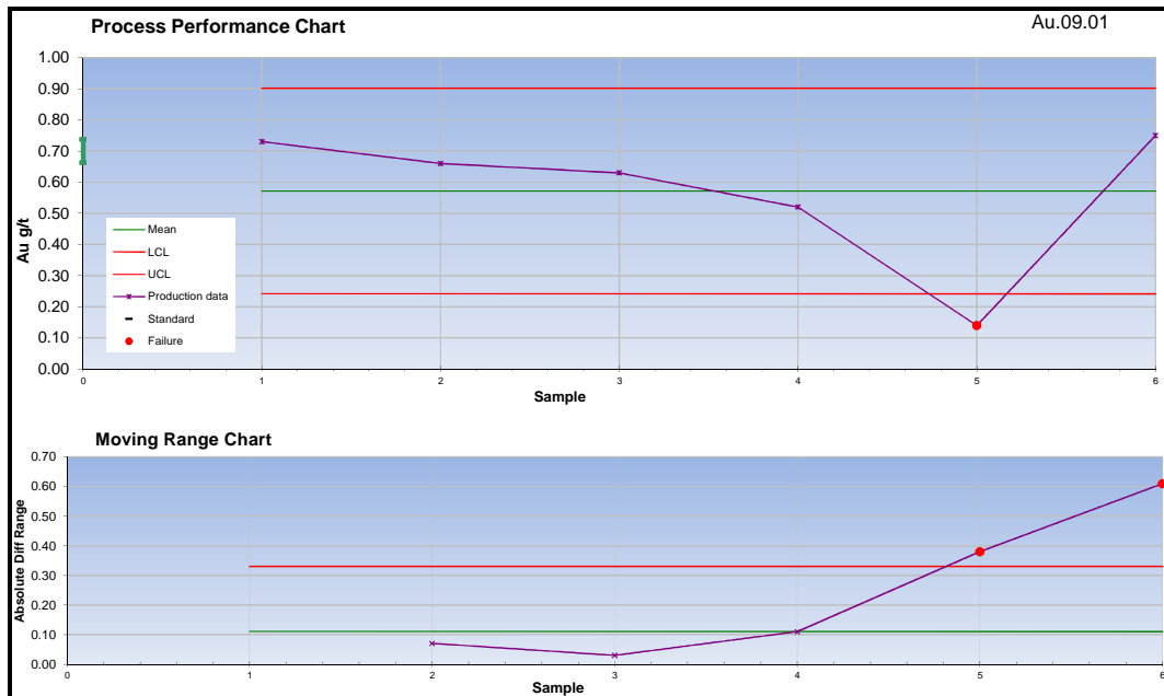
Figure 11.7 SRM Au.09.01 – Gold Plot
