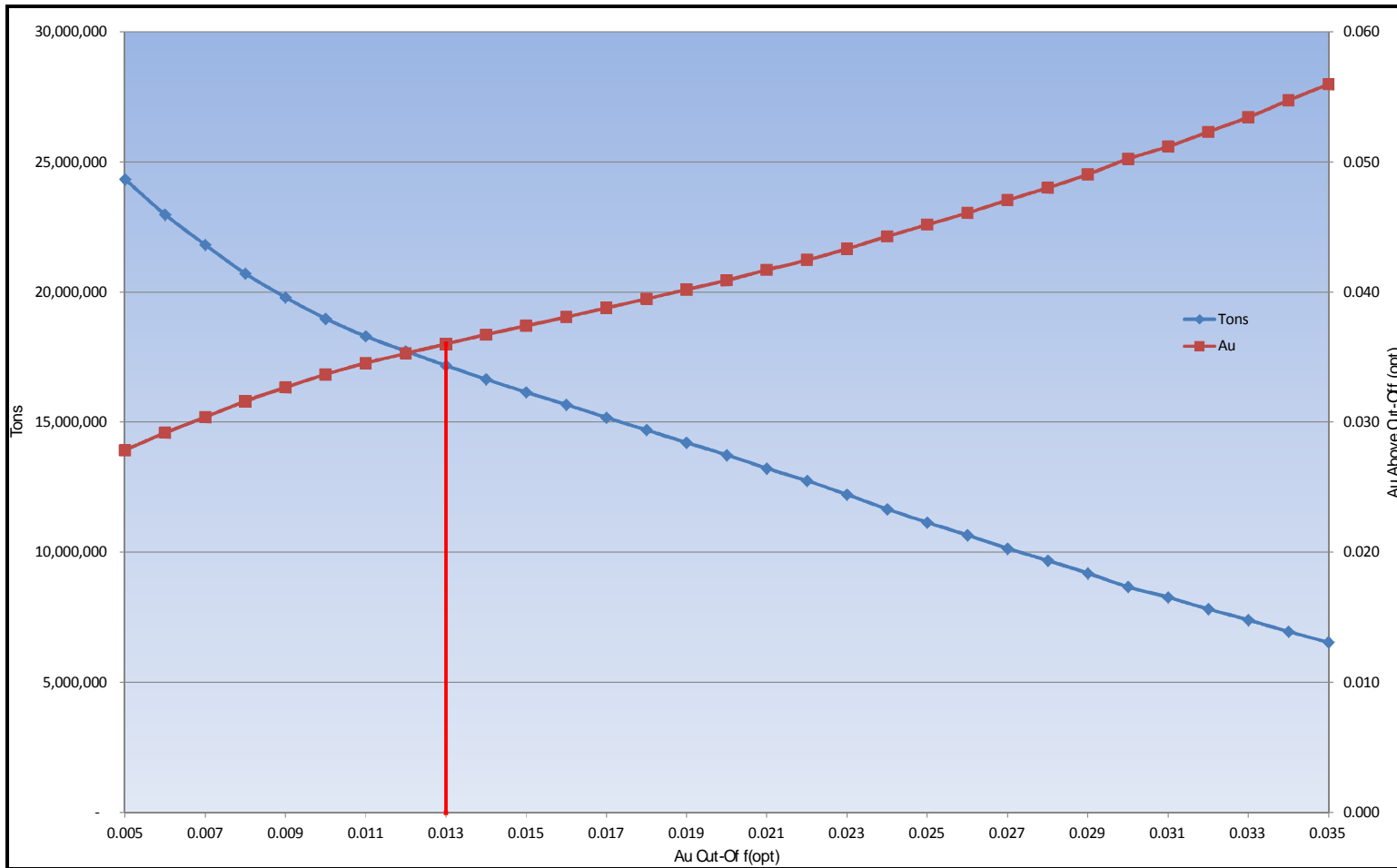
Figure 14.43 Talapoosa Measured Grade-Tonnage Curve
