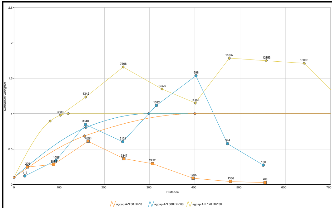
Figure 14.27 Main Vein Silver Variogram
