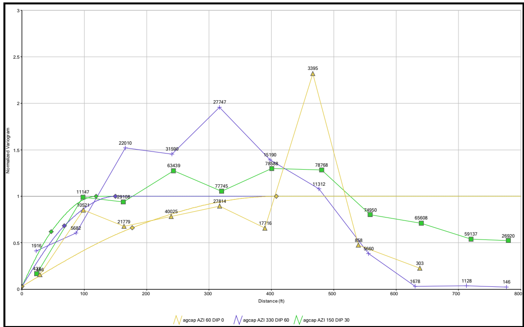
Figure 14.35 Bear Creek Footwall Zone Silver Variogram
