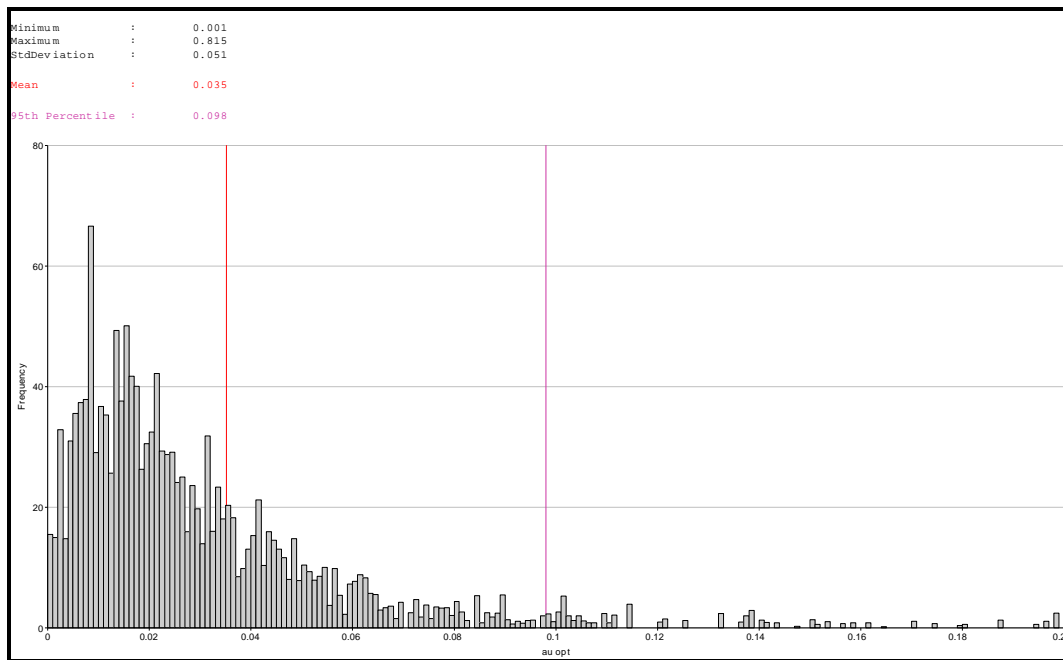
Figure 14.13 Bear Creek Footwall Vein Gold Histogram Plot
