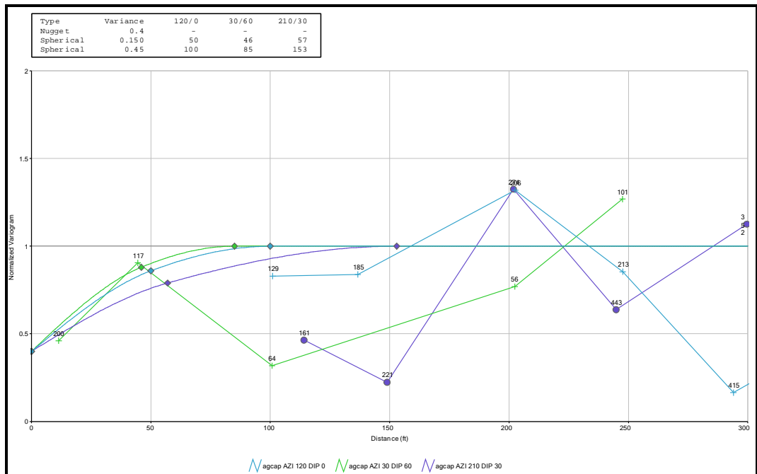
Figure 14.29 Dyke Adit Vein Silver Variogram
