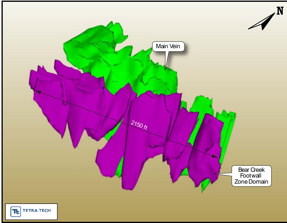
Figure 14.3 Oblique View Bear Creek Footwall Vein
