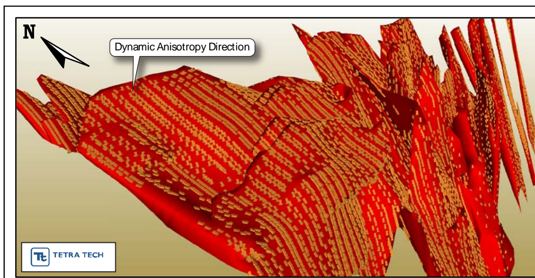
Figure 14.42 Dynamic Anisotropy Direction
