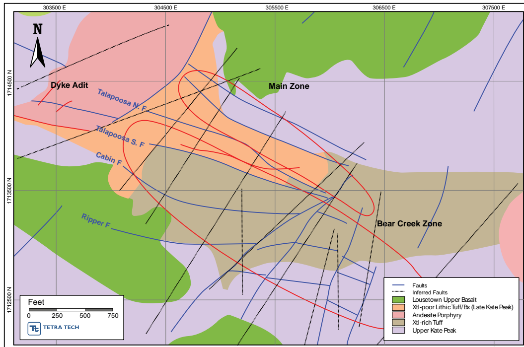
Figure 7.2 Project Geology
