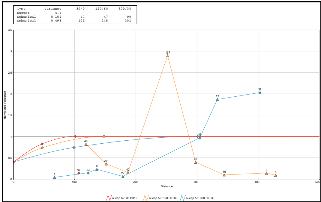
Figure 14.30 East Hill Vein Gold Variogram
