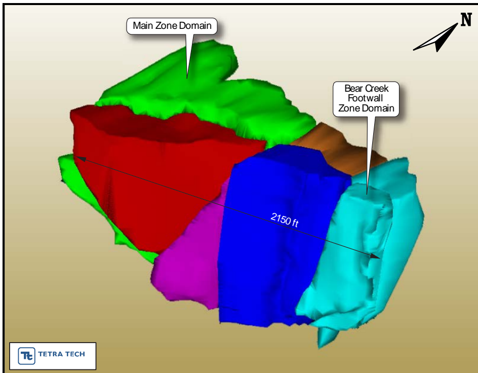
Figure 14.8 Oblique View Bear Creek Footwall Zone
