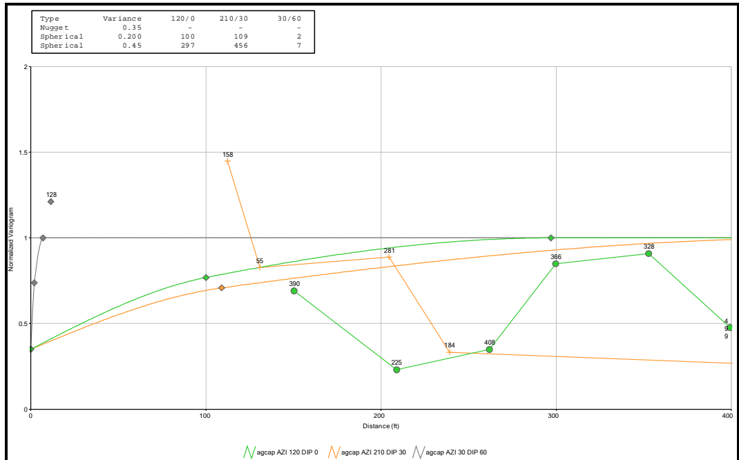
Figure 14.31 East Hill Vein Silver Variogram
