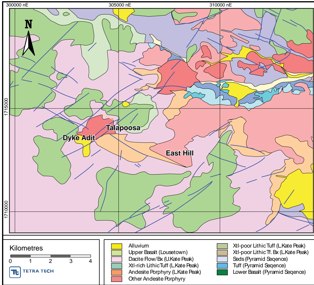
Figure 7.1 Regional Geology
