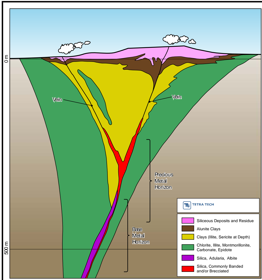
Figure 8.1 Epithermal Model
